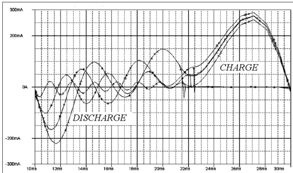
Figure 5. Pulse charge-discharge device PSpice model multi variant study results
