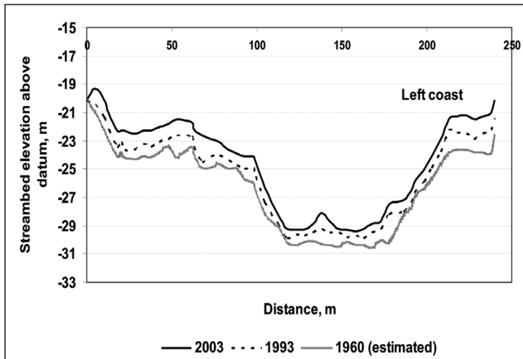
Figure 3. Rising of the riverbed at Salyan over the period 1960-2003
