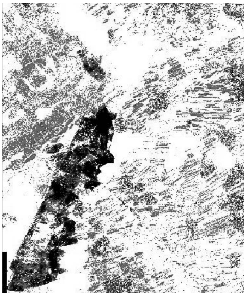
Figure 2. Unsupervised classification (black zone – area of fire).
