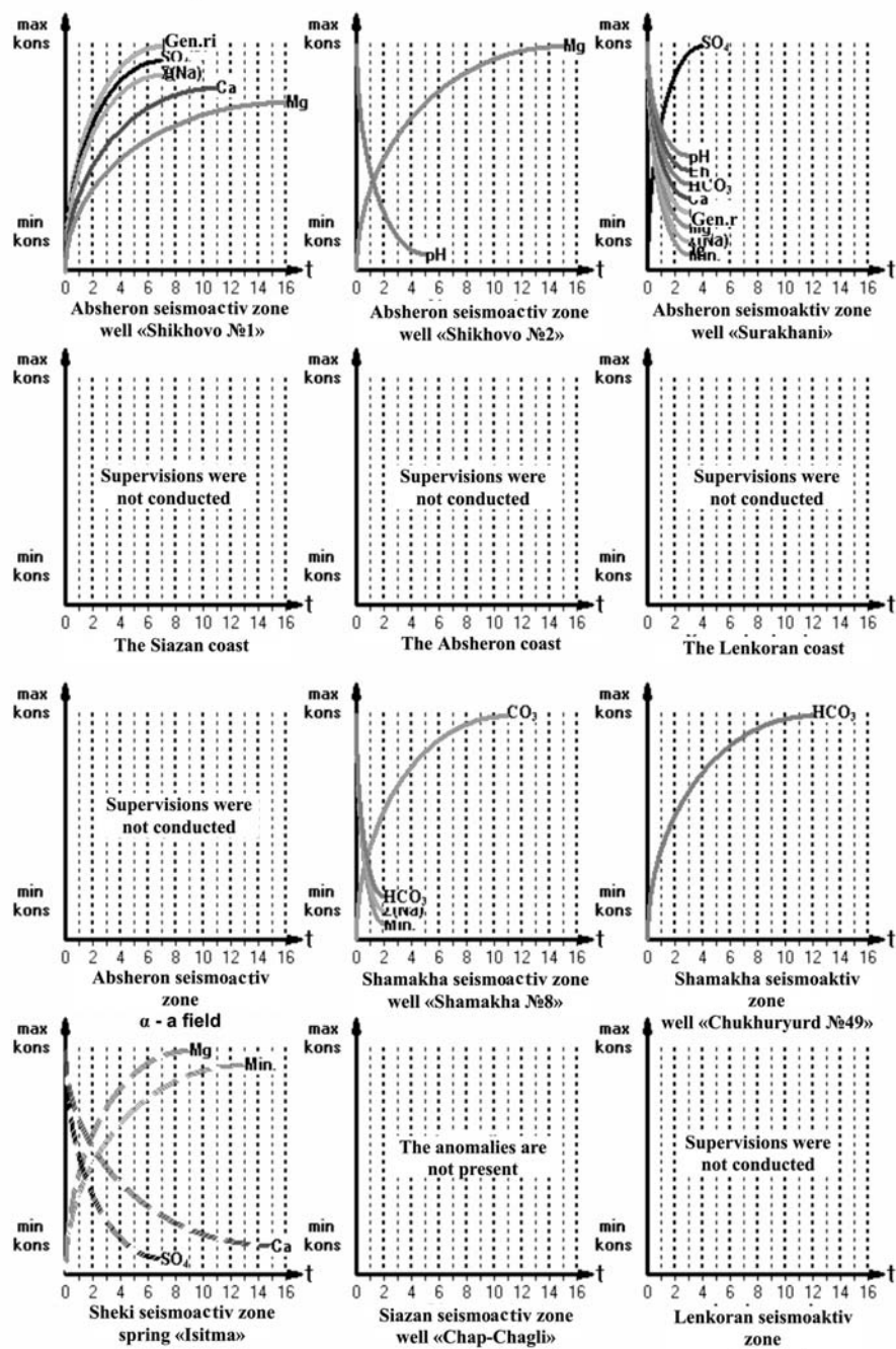
Figure 1. Identification figure – geochemical “portrait” of the seismic center
