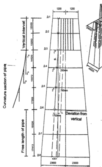
Fig.1.-Oriented location for marine stationary platform - 9 and directional hole azimuth
