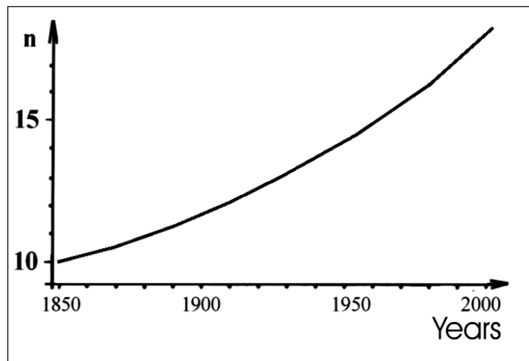
Figure 7. The trend of the volcanic activity
