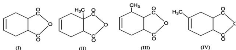
Figure 2. Molecule of anhydride BHDA
