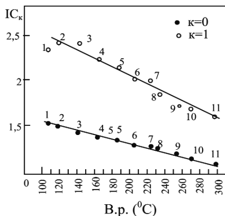
Figure 3. Dependence of change of index IC_k ( k = 0, 1 ) on B.p. ( ^{\circ}C ) of monocarboxylic acids of C_1 - C_{12} of paraffin series
