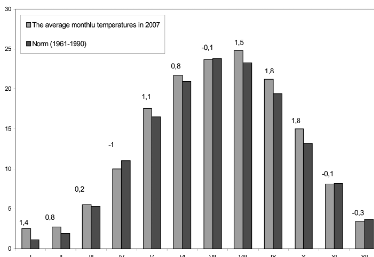
Figure 1. Comparing of 2007 and long-term monthly values (1961-1990) of temperature
