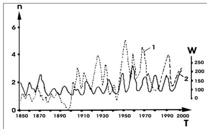
Figure 3. Comparison of solar and mud (M) volcano activities diagrams.
