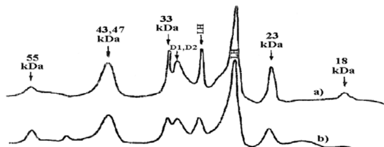
Figure 3. Densitogramme of protein spectrum of subchloroplasts particles PS2; a) control; b) irradiated ( 4 \cdot 10^7 \text{ erq/sm}^2 ).
