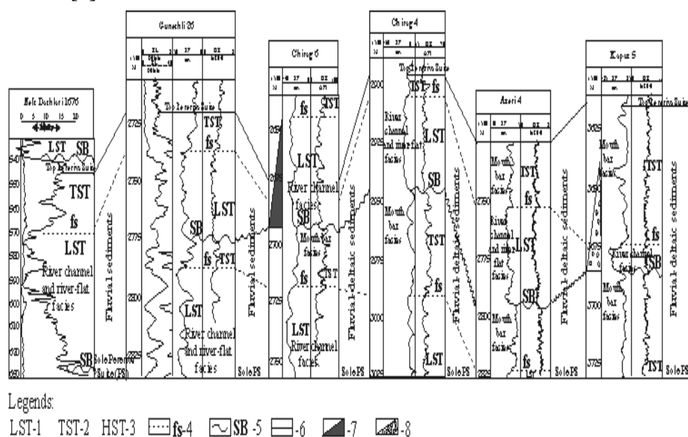
Figure 2. Correlation profile of the Pereriva Suite deposits of the Productive Series of Absheron-Pribalkhanskiy uplift zone:
